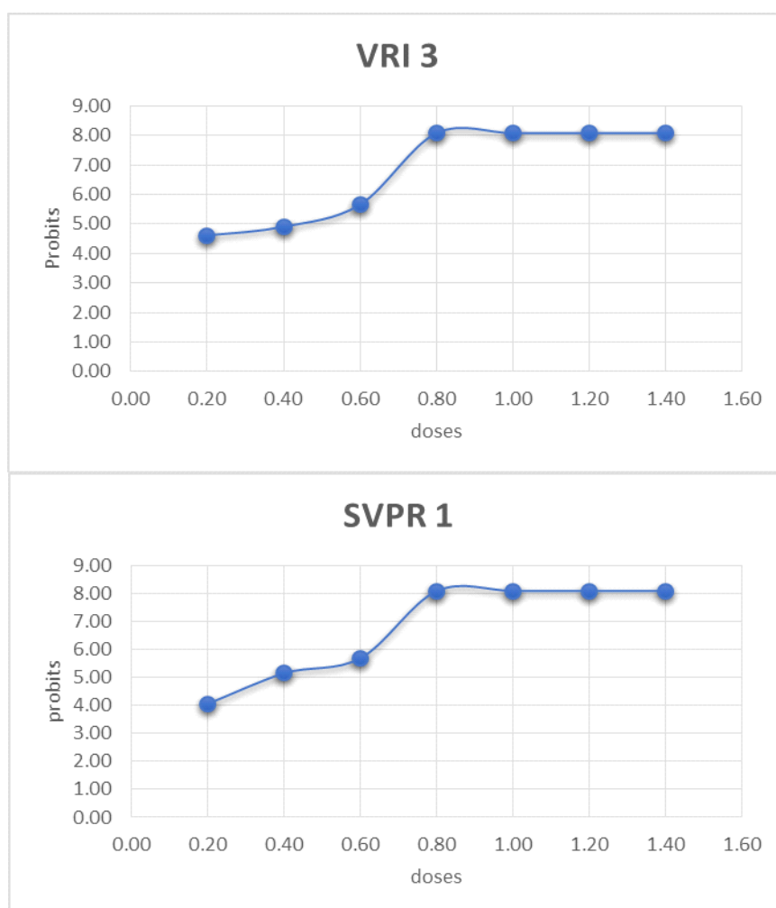
Fig. 1. Plots of Mutagenic Doses vs Probits for Calculation of LD50 of EMS in VRI 3 and SVPR 1
