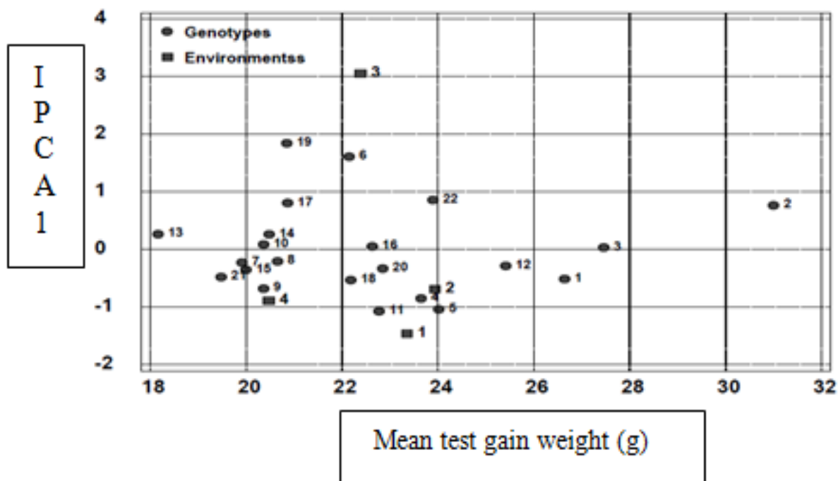
Fig 3: AMMI 1 biplot of test grain weight showing main effects and G x E interaction of rice genotypes in four environments
