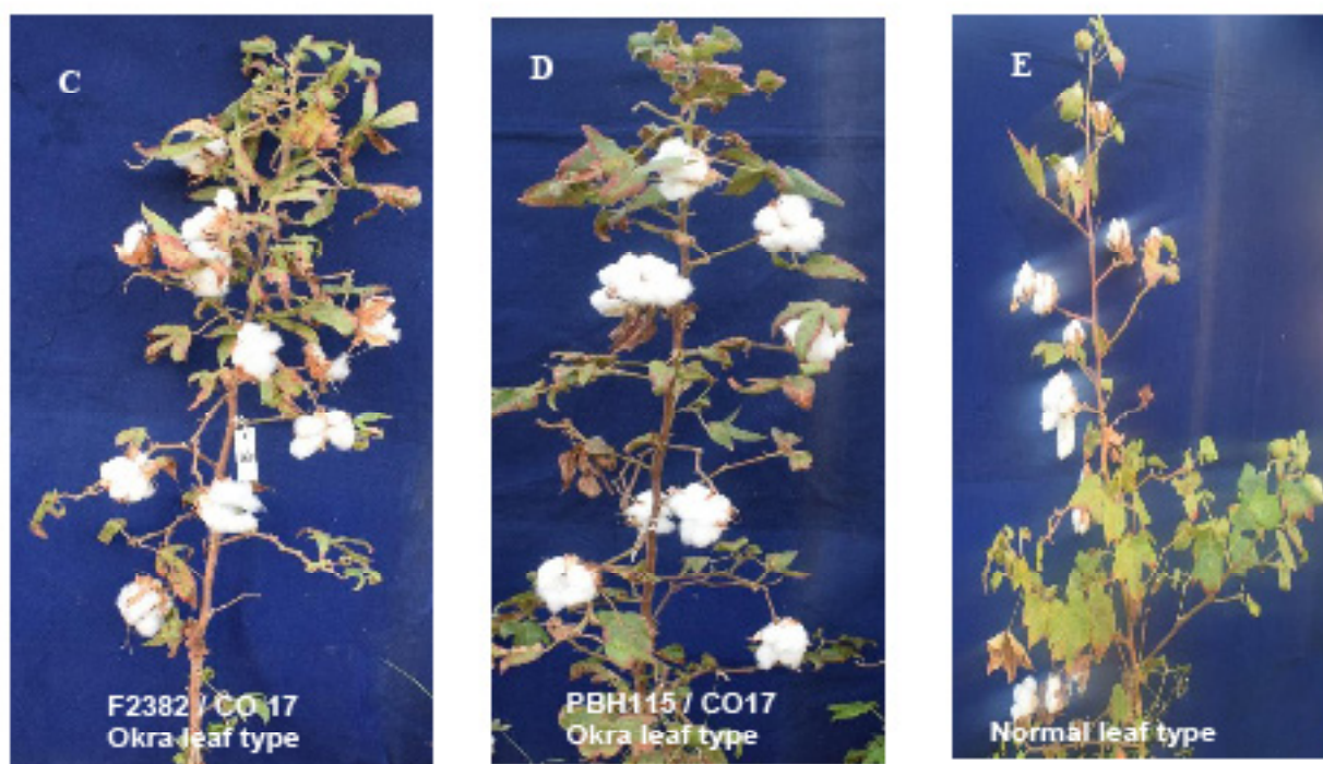
Plate 2. Comparison of Normal leaf (E) with okra leaf type of F2382/CO17(C) and PBH115 /CO17 (D)
