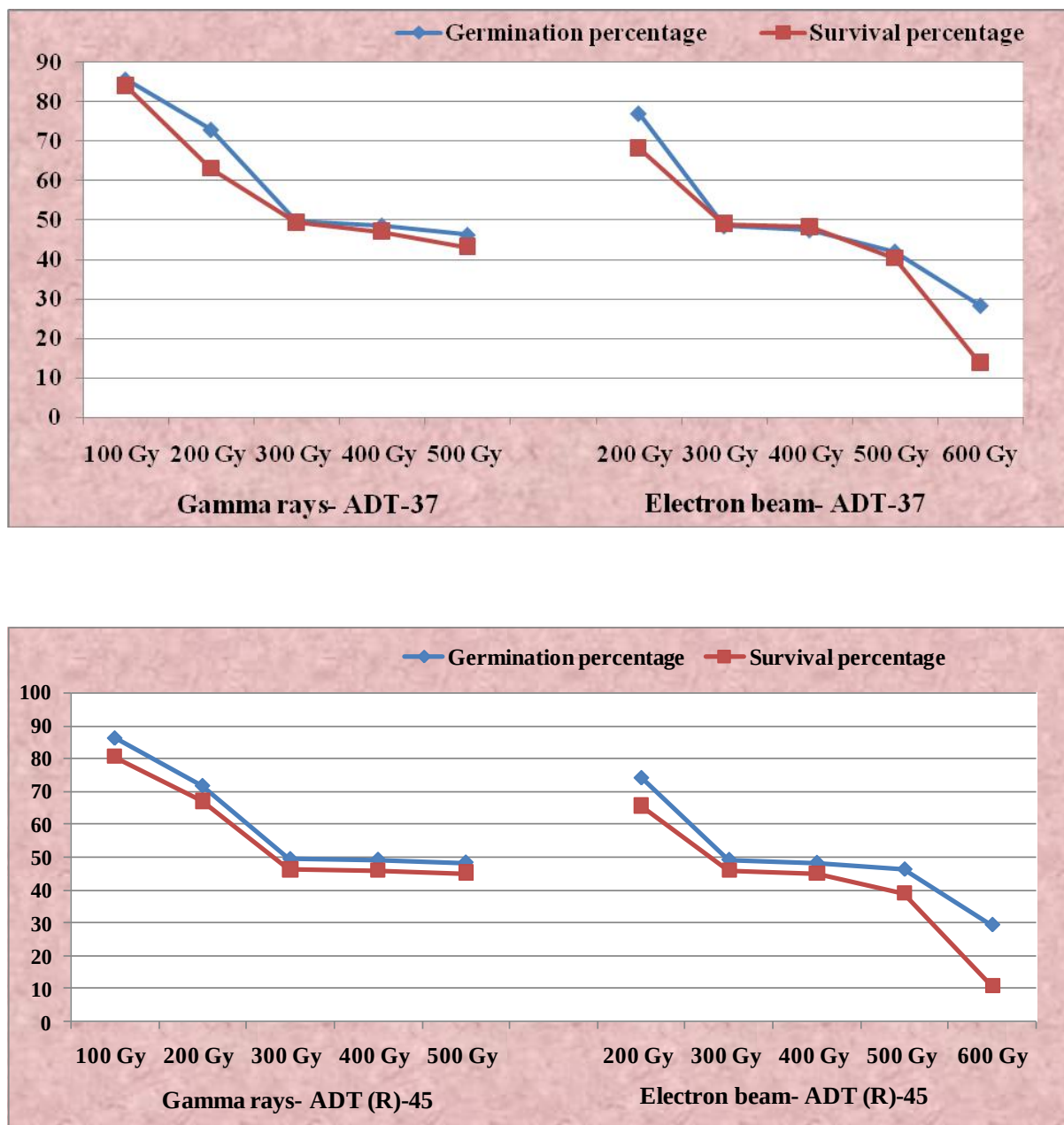
Fig 3. Comparison of germination percentage and survival percentage reduction over control at different doses of gamma rays and electron beam in ADT-37 and ADT(R) 45
