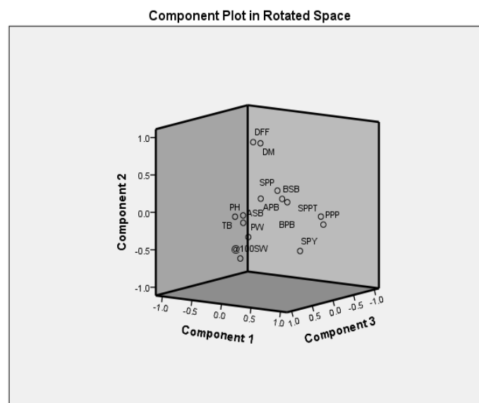
Figure 2. Three dimensional component plots for 14 quantitative traits in chickpea germplasm
