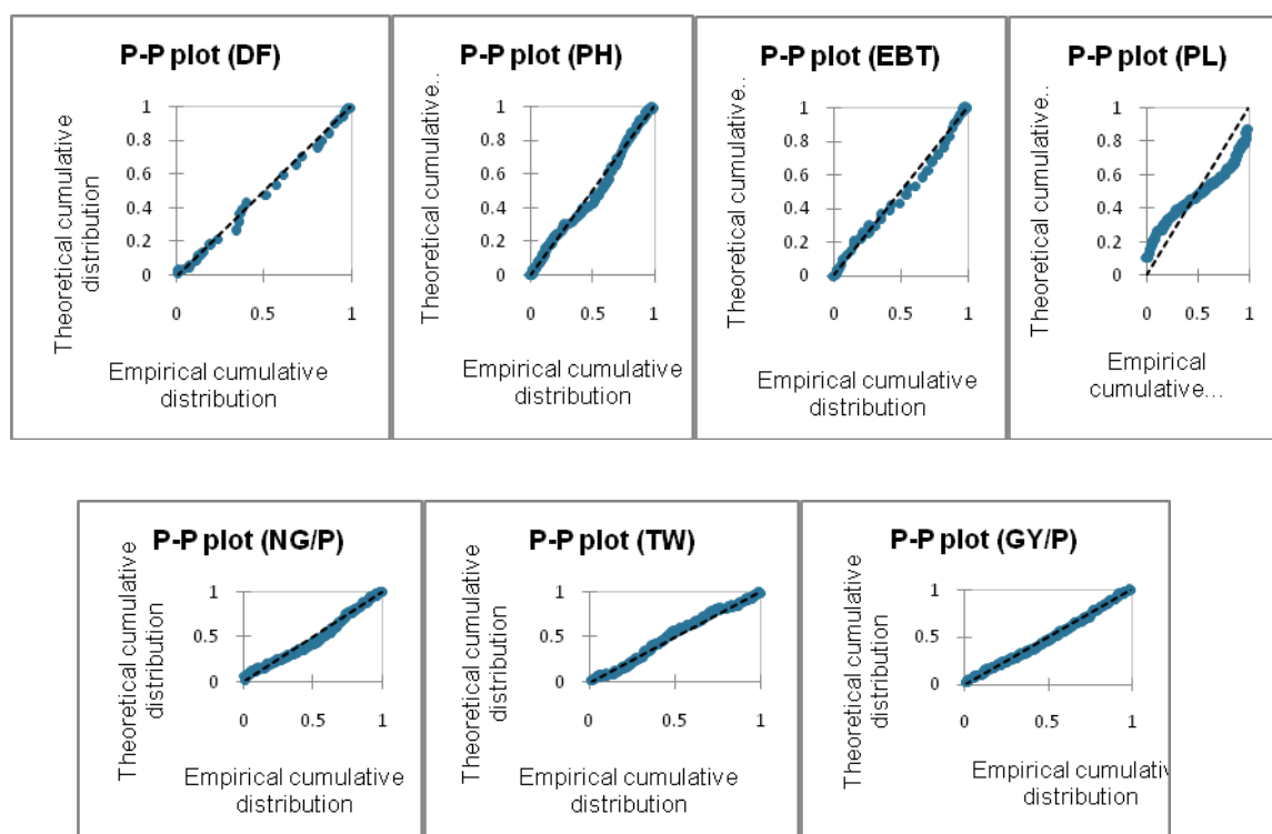
Fig. 2. Normal p-p plots depicting variation in all 7 quantitative characters of rice genotypes
