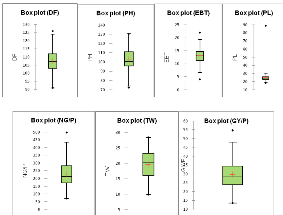
Fig. 1. Box-plots depicting the variation of the data from 217 rice accessions. Dots sketch outliers
