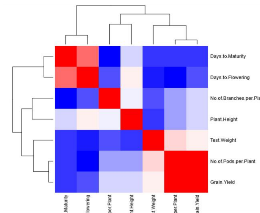
Fig. 3. A heat map of horse gram germplasm accessions showing the relationships between yield and yield related traits.
