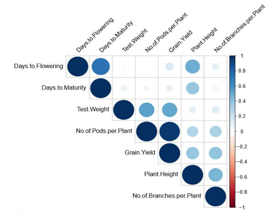
Fig. 1. Correlation Matrix showing character's correlation with each other. A positive correlation is shown in blue and negative correlations in shown in red color. The color intensiveness and the size of the circle are relatively proportional to the correlation.
