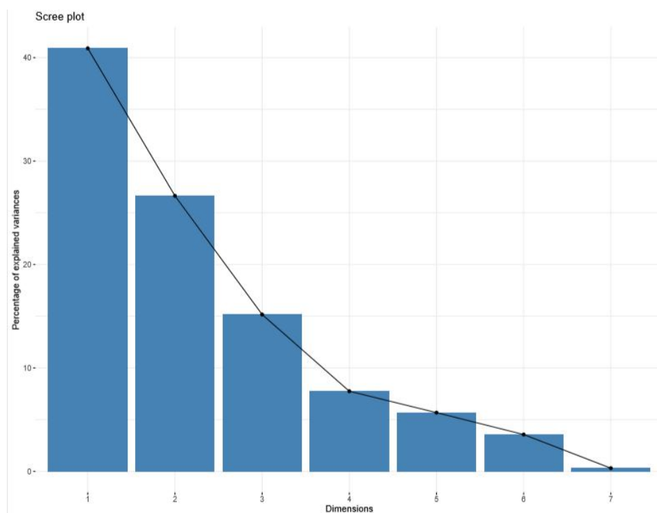
Fig. 6. Screen plot showing variance and along with Principal components
