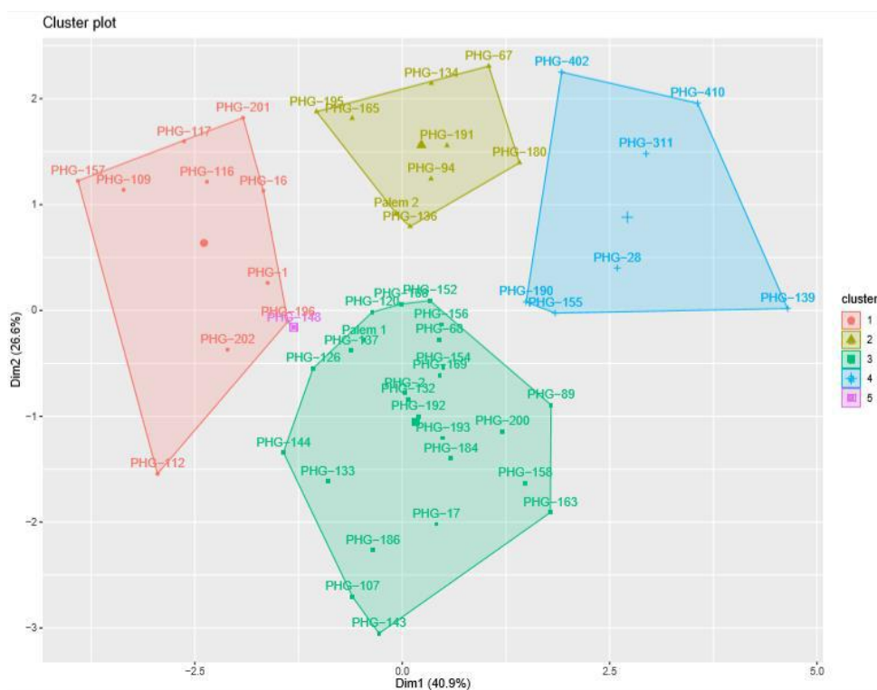
Fig. 4. K-means clustering pattern of genotypes (k=5)
