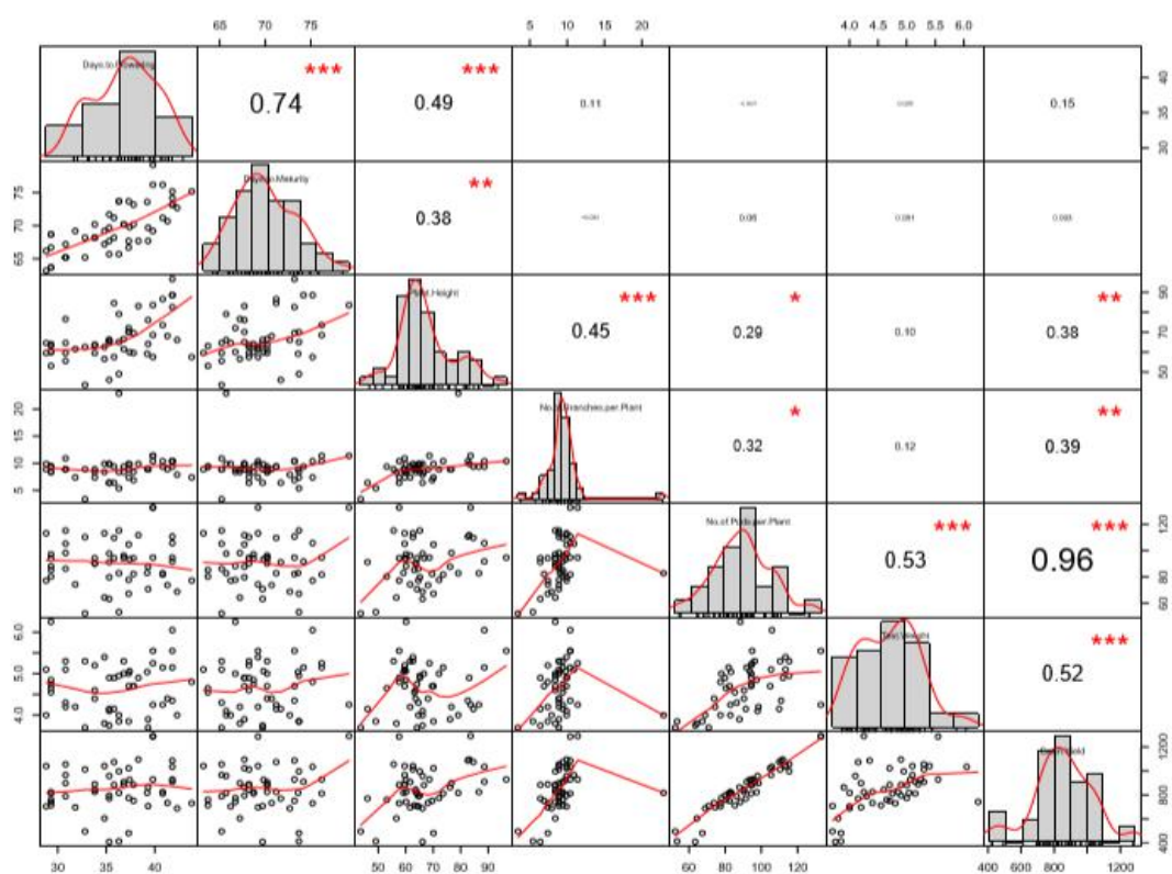
Fig. 2. Schematic model of plot showing the significance of traits with each other as well as other traits
