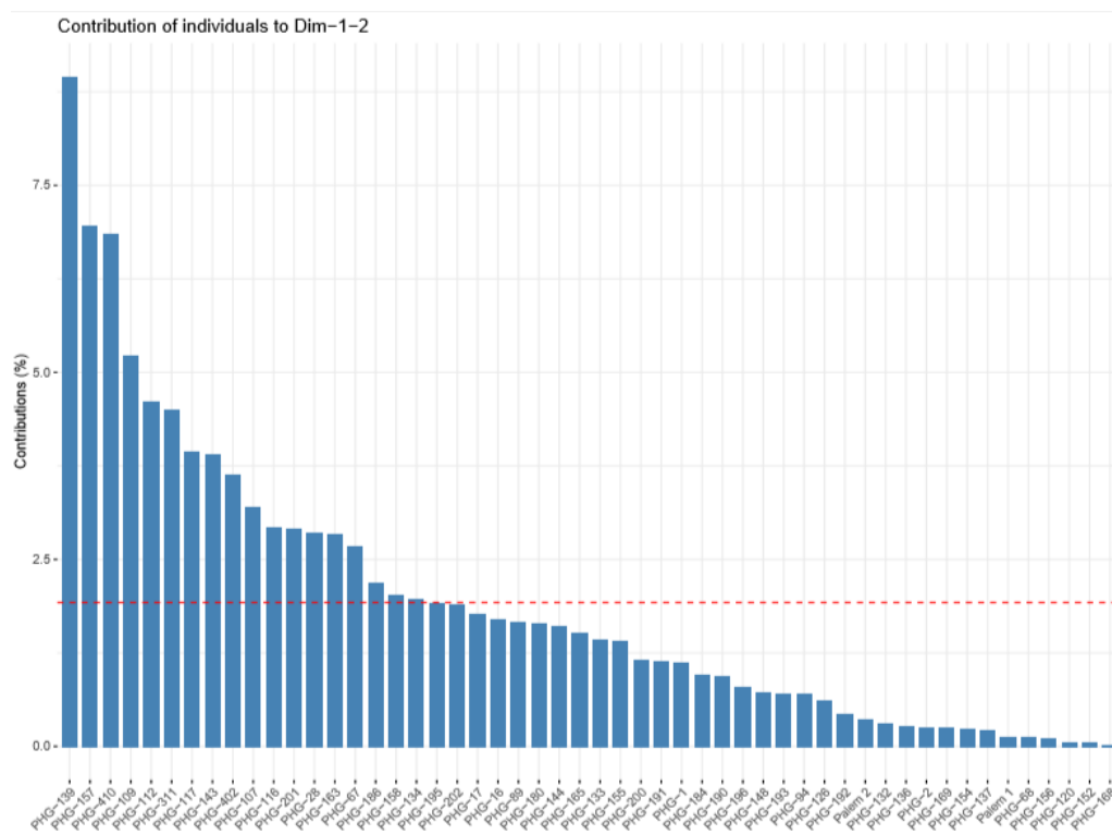
Fig. 8. Contribution of genotypes to dimensions 1 and 2
