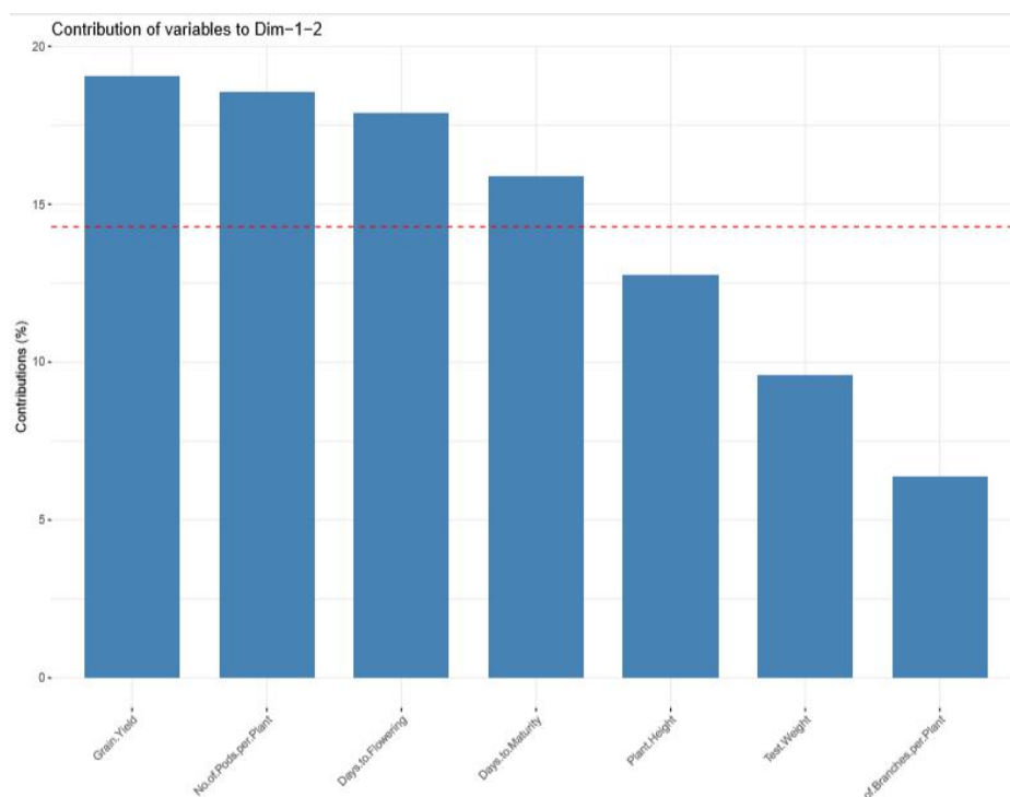
Fig. 7. Contribution of traits to dimensions 1 and 2
