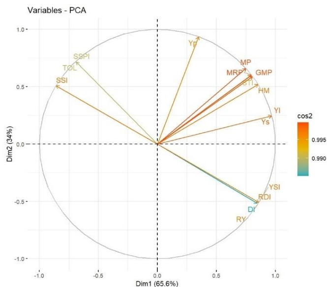
Fig. 3. Biplot showing proportion of contribution of the traits and their association in the principal components under drought condition
