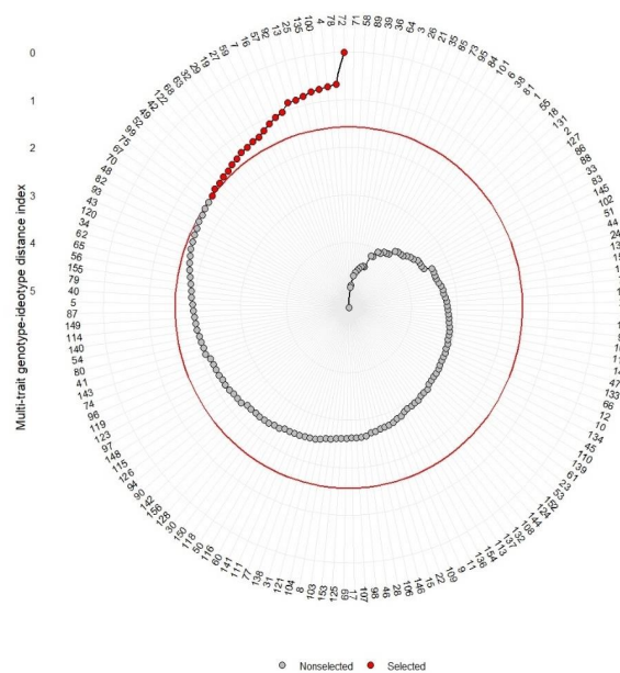
Fig. 2. The rankings of sorghum germplasm lines illustrate the selected accessions based on the multi-trait genotype–ideotype index (MGIDI). Selected lines are indicated by red dots, while unselected accessions are represented by grey dots. The red circle denotes the cutoff point determined by the selection pressure
