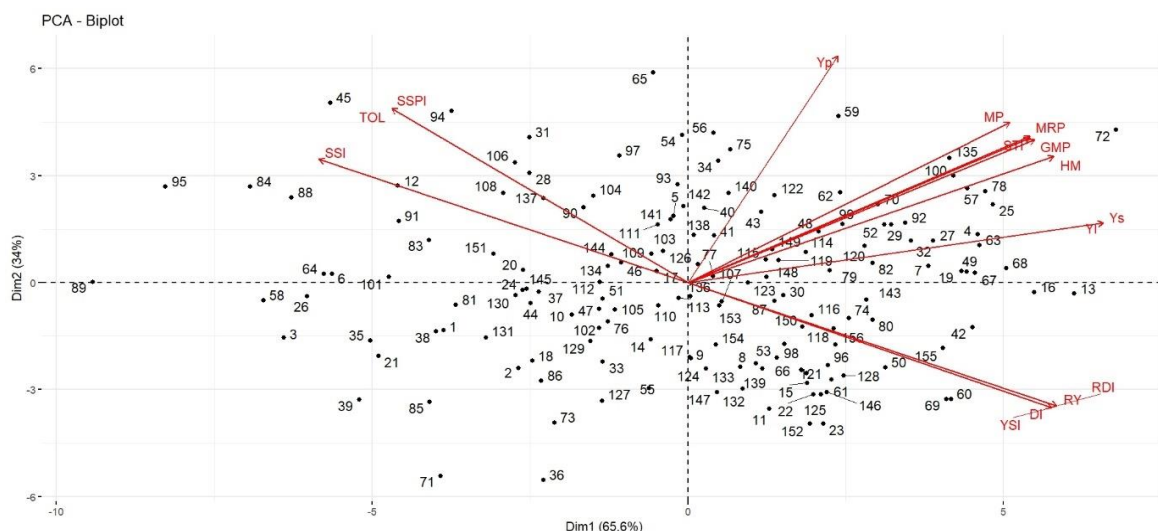
Fig. 4. PCA Biplot between PC1 and PC2 derived from PCA analysis showing distribution of sorghum germplasm lines
